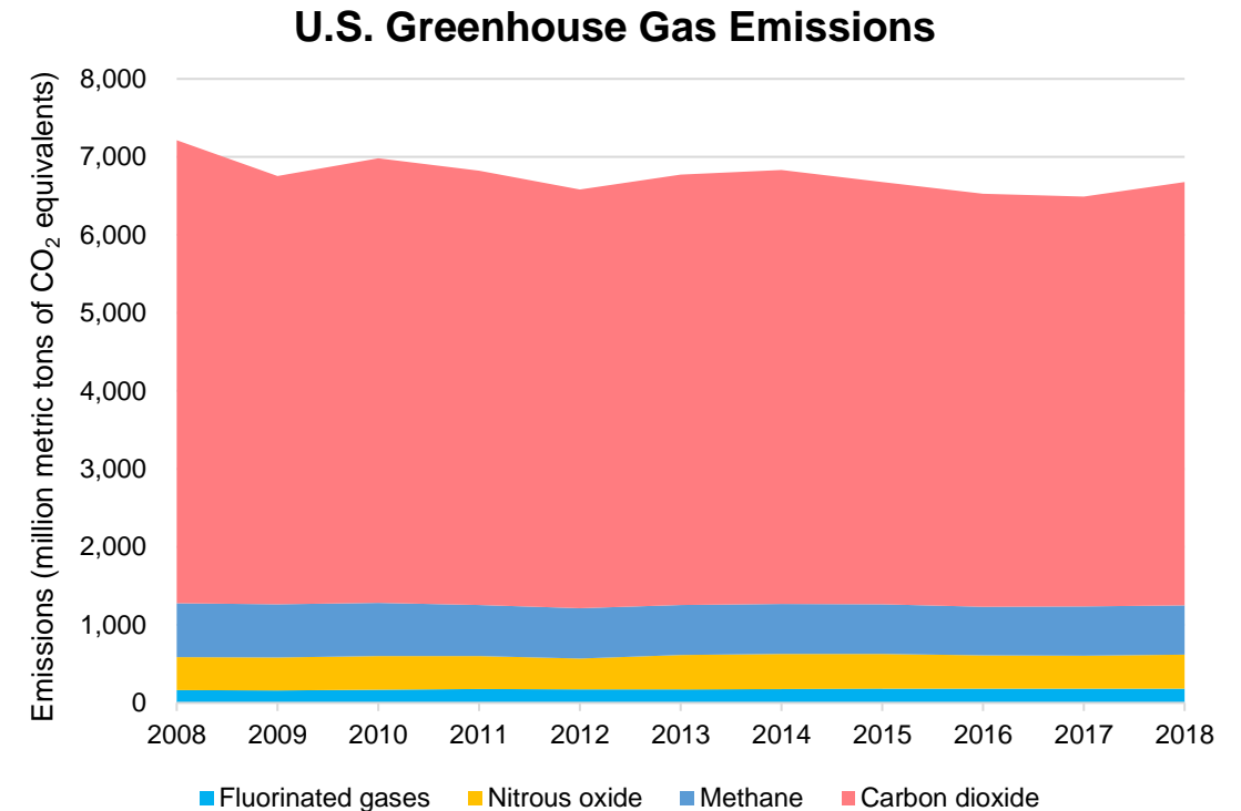
Source: U.S. EPA's Inventory of U.S. Greenhouse Gas Emissions and Sinks
